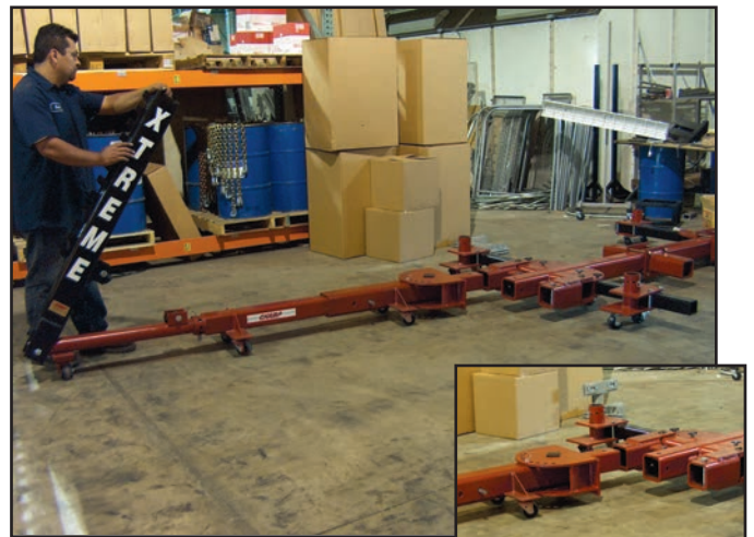
Insert assembled Pulling Tower into each of the Six tower inserts. Lock into place with Locking Pin.
